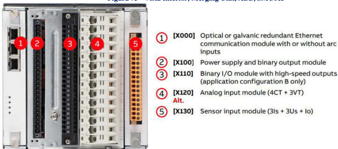
Figura 73 - Vista Interior, Merging Unit, ABB, SMU615
